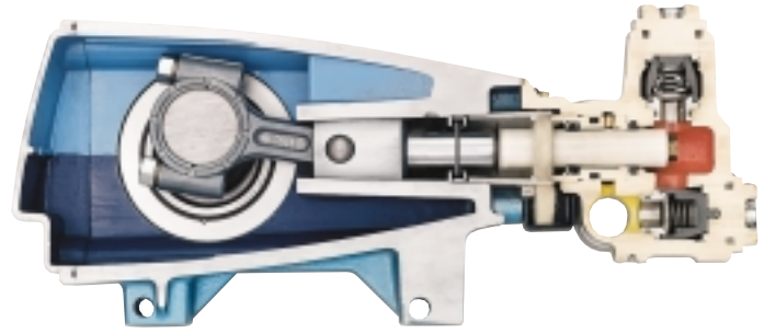
Plunger Pumps
